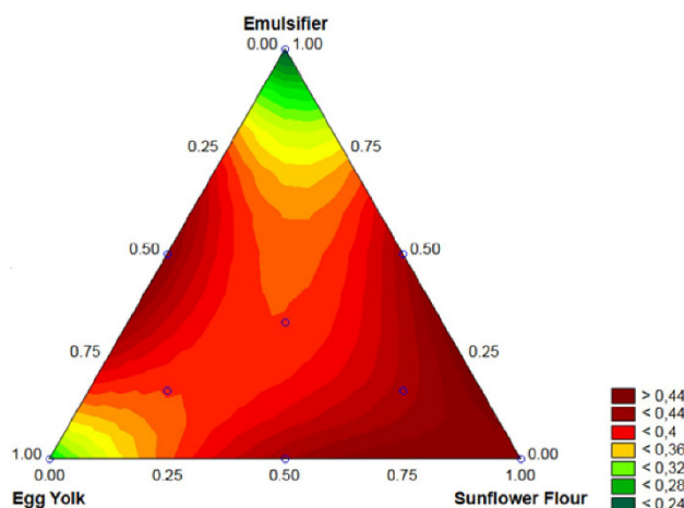
Figure 2. Effect of the addition of reconstituted egg yolk powder (EYP), de-oiled sunflower meal (DSF) dispersion and DATEM emulsifier (E) on water activity.
